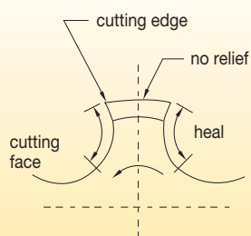
Concentric
