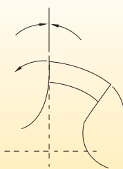
Radial Rake
